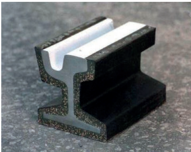
Factory Pre-Coated Rail
