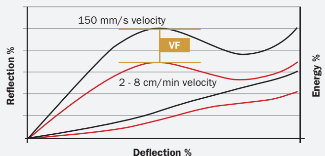
VF: ratio of reaction force at berthing speed and testing speed
