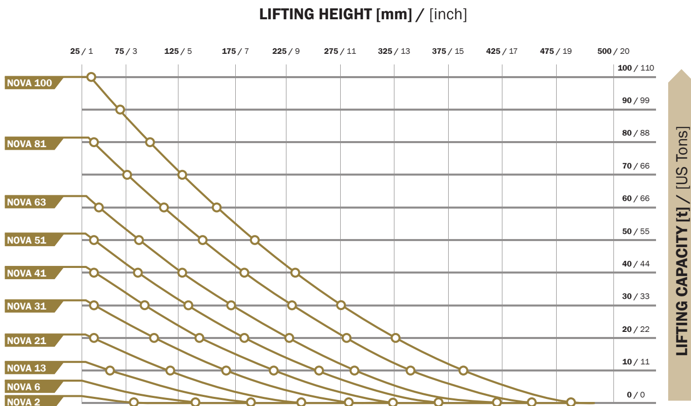
Graph 3: Lifting characteristics of NOVA high-pressure lifting bags
