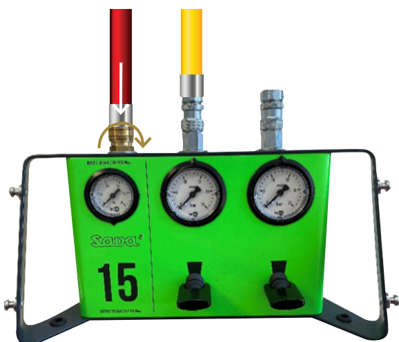
Figure 7.12: Connecting the inflation hose to the controller.
