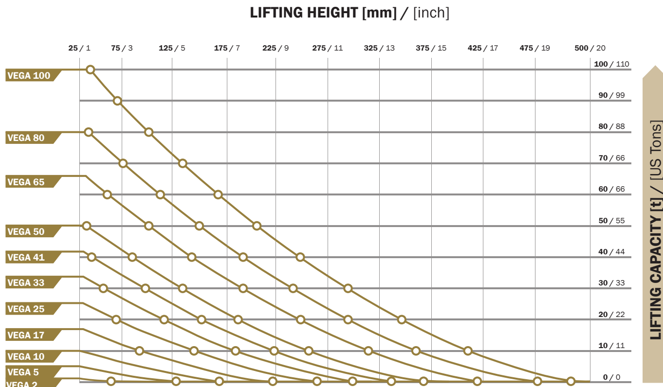
Graph 1: Lifting characteristics of VEGA high-pressure lifting bags
