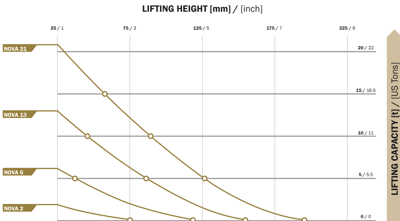
Graph 4: Lifting characteristics of NOVA 2, NOVA 6, NOVA 13 and NOVA 21 high-pressure lifting bags
