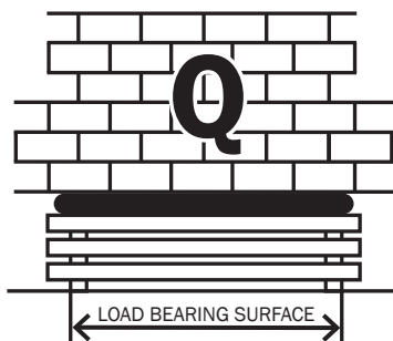
Figure 7.17: Substructure support and the bearing surface.
