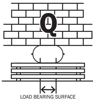
Figure 7.19: Minimum load-bearing surface at maximum lifting height.
