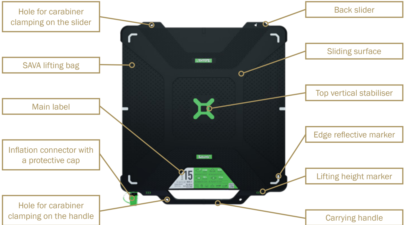
Figure 6.1: Description of SAVA lifting bag.
