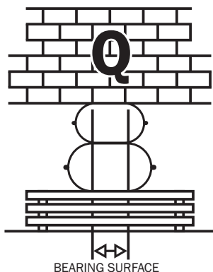
Figure 7.23: Combination of two SAVA lifting bags to increase the lifting height.
