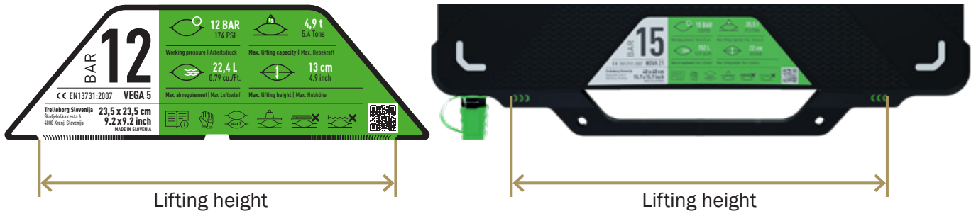
Figure 6.3: Graphically illustrated lifting height of VEGA and NOVA high-pressure lifting bags.
