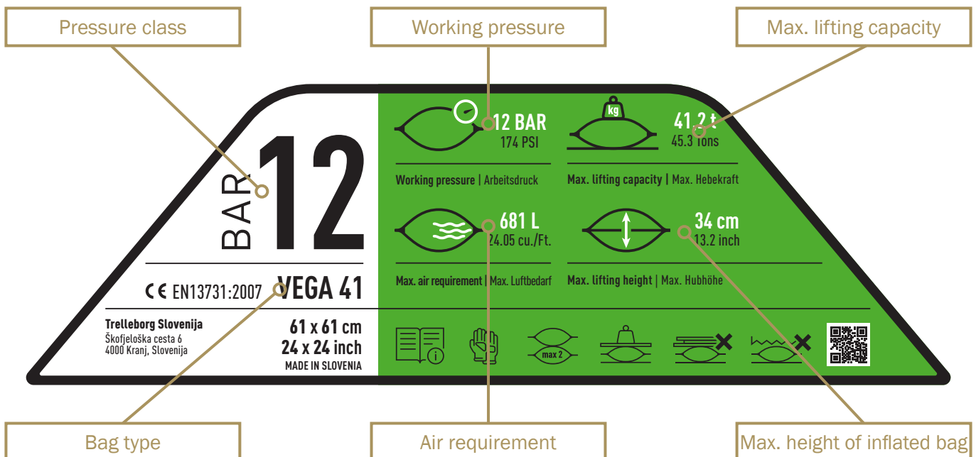
Figure 6.2: Bag label data explanation.
