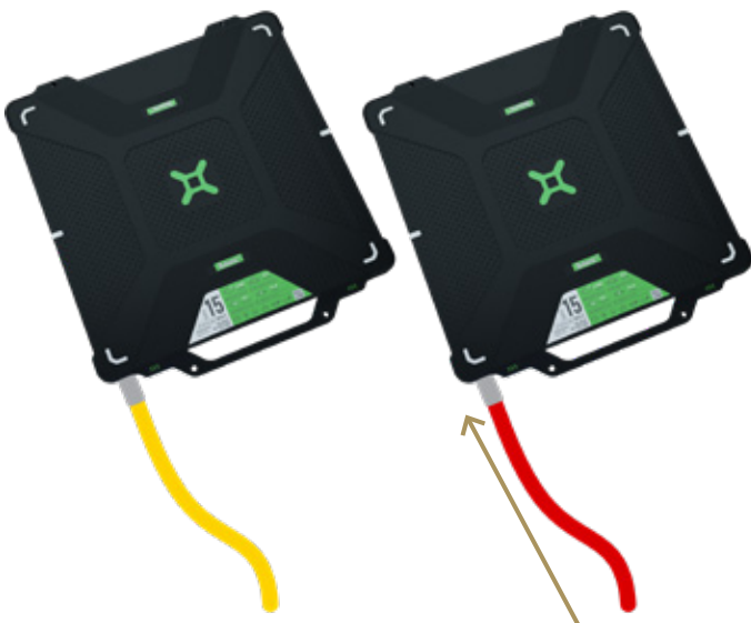
Figure 7.7: Connecting the hose to SAVA lifting bag.
