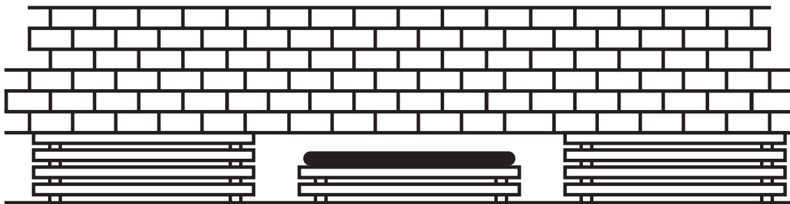
Figure 7.20: Construction of safety supports – non-inflated lifting bag.
