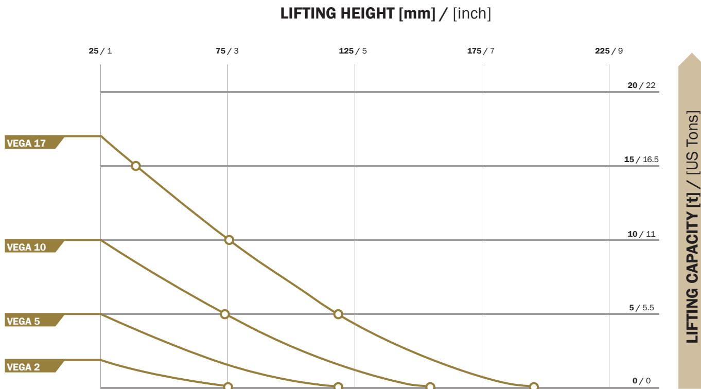
Graph 2: Lifting characteristics of VEGA 2, VEGA 5, VEGA 10 and VEGA 17 high-pressure lifting bags
