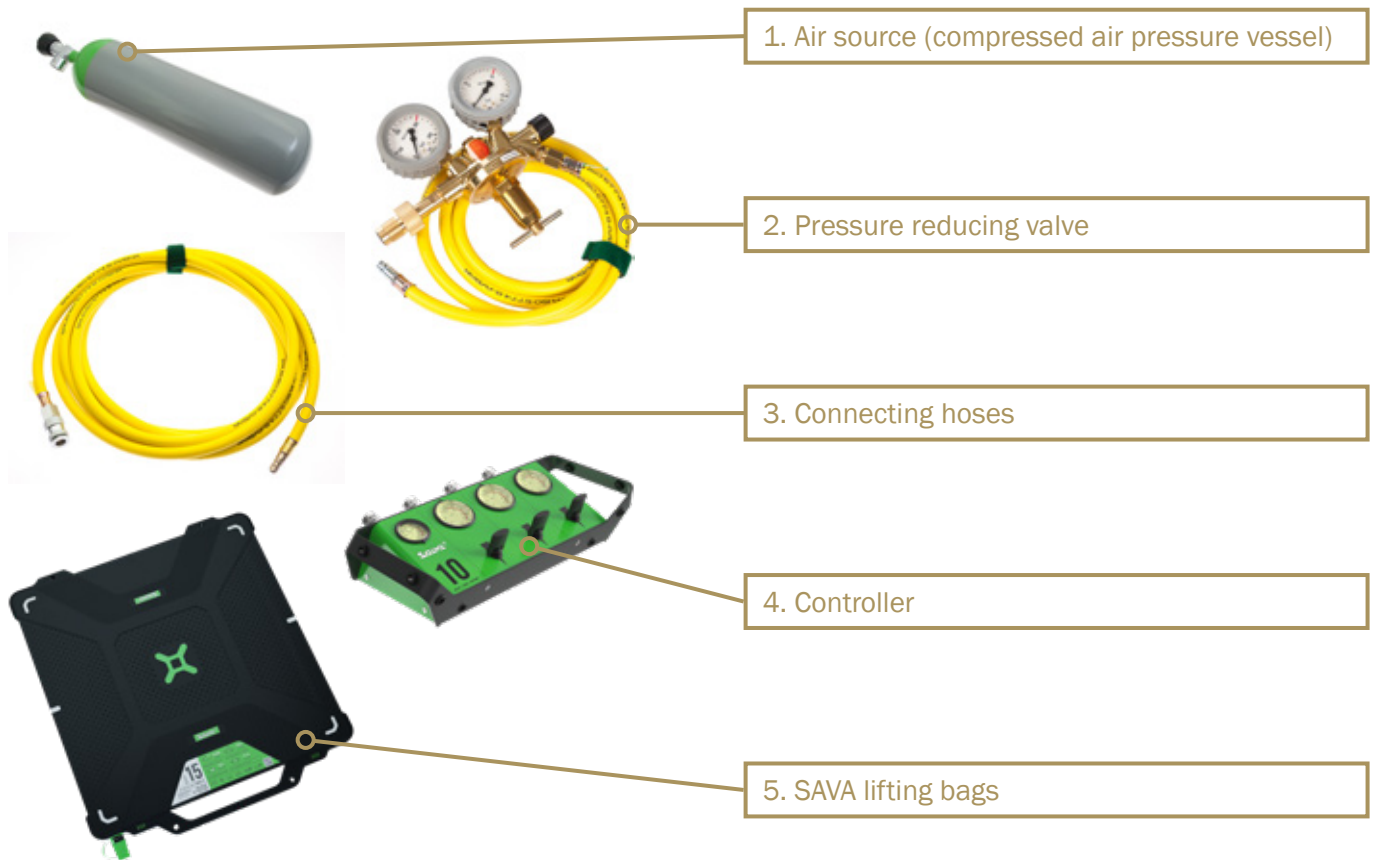
Figure 7.1: Components of the load lifting system with SAVA lifting bags.
