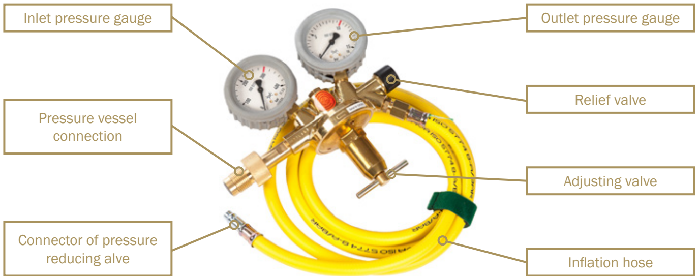
Figure 7.2: Pressure reducing valve.
