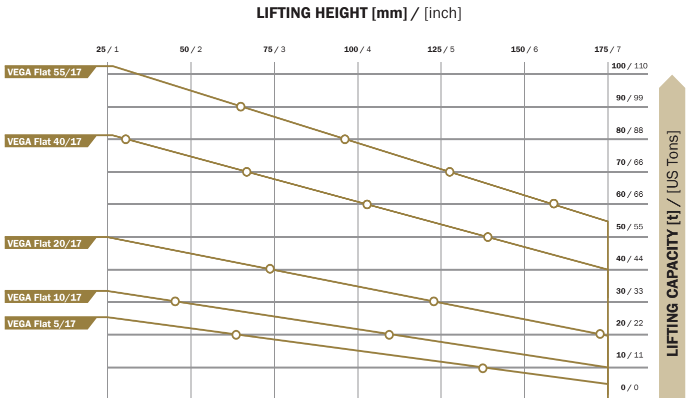
Graph 1: Lifting characteristics of high-pressure flat lifting bags VEGA Flat
