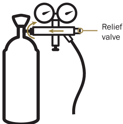
Figure 7.10: Installing the pressure reducing valve.
