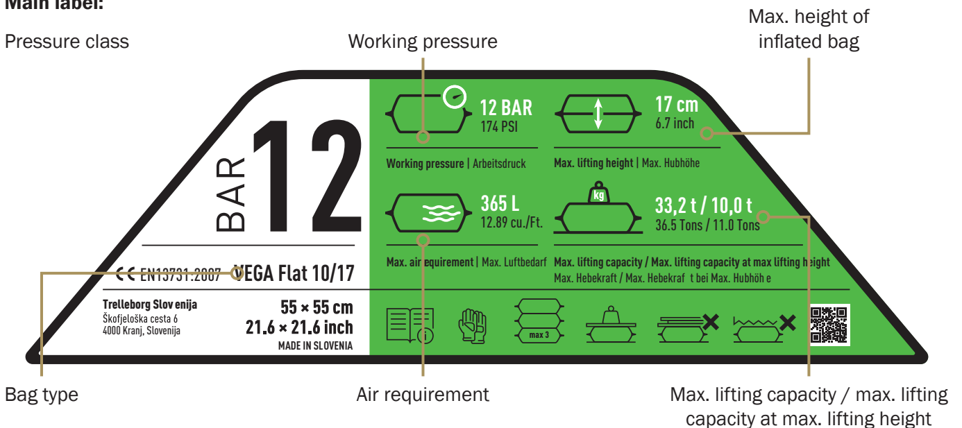
Figure 6.2: Explanation of bag label data
