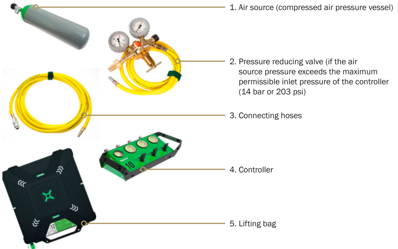
Figure 7.1: Components of the load lifting system using lifting bags.
