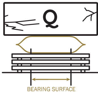
Figure 7.19: Minimum load-bearing surface at maximum lifting height.
