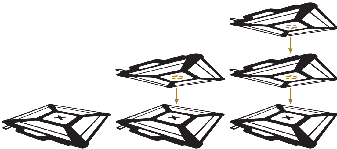
Figure 7.26: Combining flat lifting bags to increase the lifting height.
