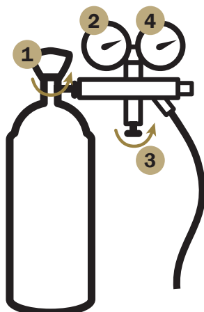
Figure 7.11: Setting the pressure reducing valve.
