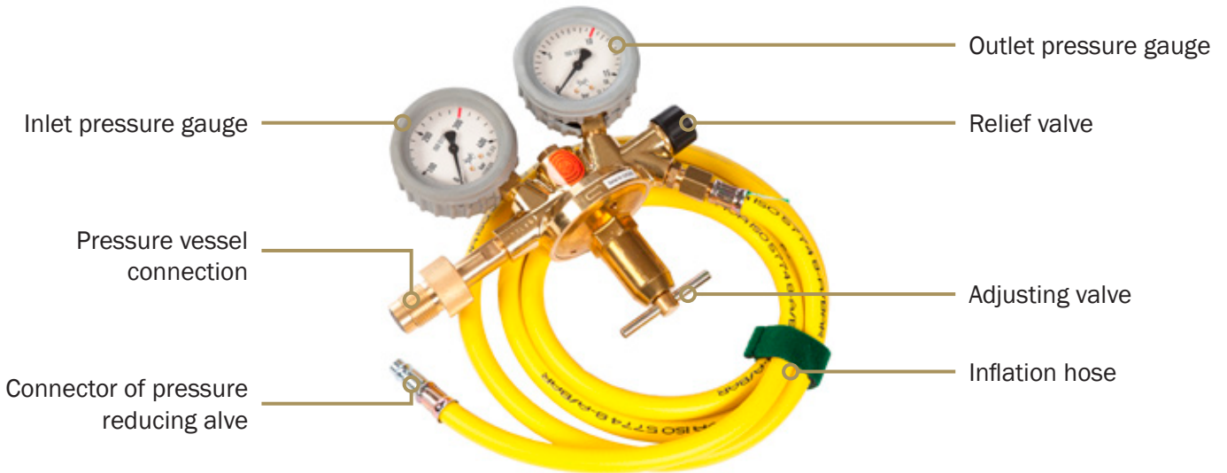
Figure 7.2: Pressure reducing valve – schematic presentation.
