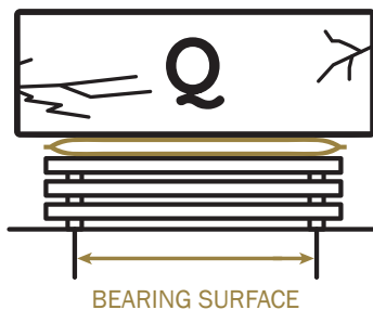
Figure 7.17: Load support structure and marked load-bearing surface
