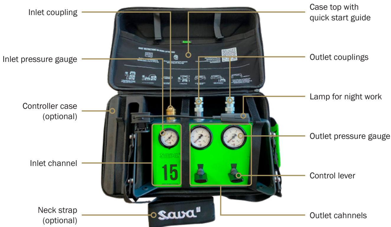
Figure 7.5: EXP controller
