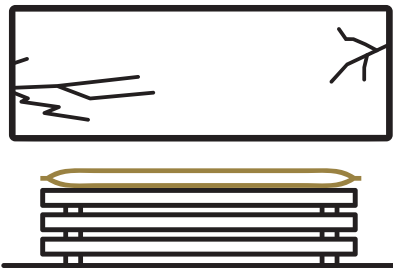
Figure 7.6: Positioning SAVA lifting bag at place of use.
